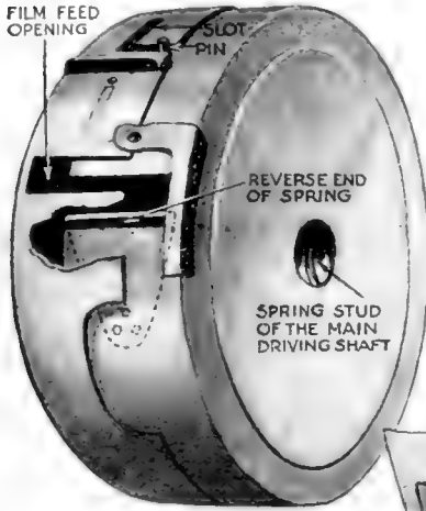
FILM BOX
